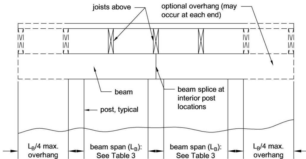
Figure 3. Beam Span.
